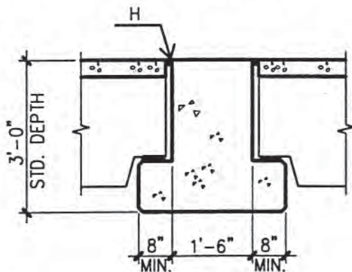
A TYPICAL SPANDREL BEAMS \frac{3}{8}'' = 1'-0'' TYP.
