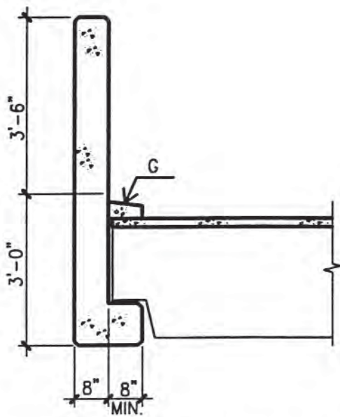
A TYPICAL SPANDREL BEAMS \frac{3}{8}'' = 1'-0'' TYP.
